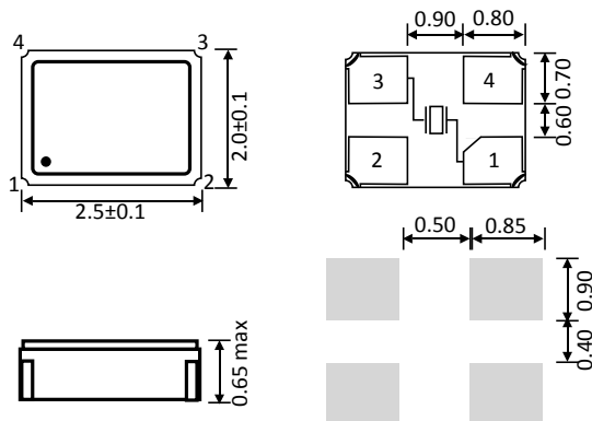
Dimensions (mm)
