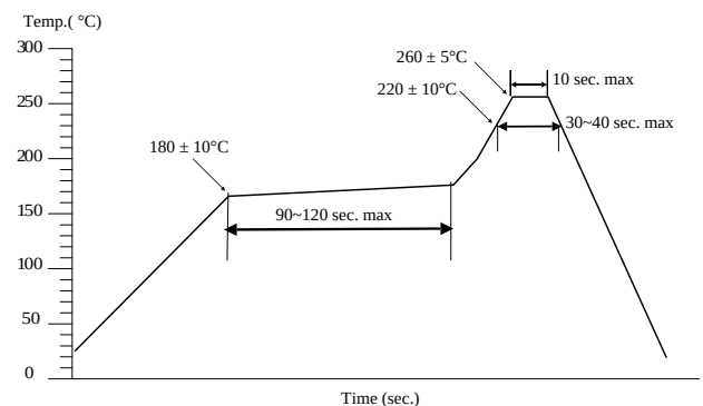
Reflow profile
